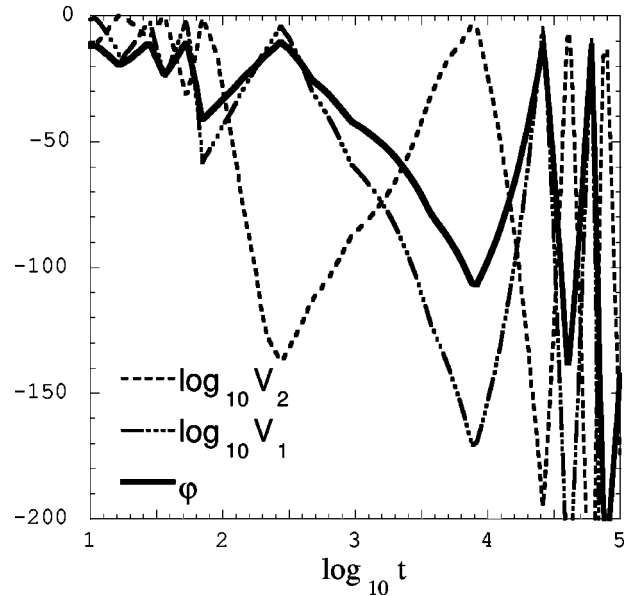
FIG. 4. New solution as an inhomogeneous U(1) -symmetric cosmology. As in previous studies of generic U(1) -symmetric cosmologies, \varphi = \gamma_g , V_1 , and V_2 are shown at a typical spatial point.
