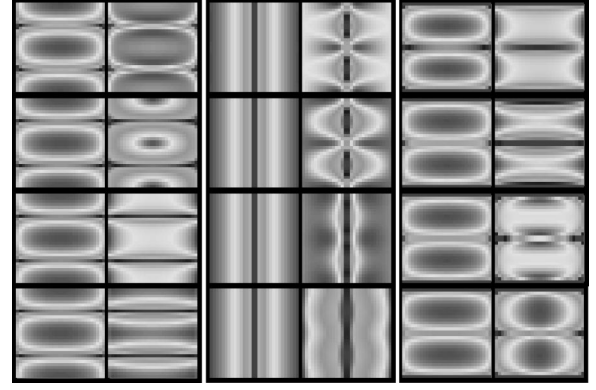
FIG. 5. Evidence for the spatial inhomogeneity of the new solutions. The spatial dependence of \gamma and \gamma_g is shown for the (\cos \theta, \varphi) plane in a series of side-by-side frames arranged in three separate panels. Each pair of frames shows the spatial dependence of \gamma and \gamma_g respectively during an approximate Kasner epoch of the seed Mixmaster solution. The panels are grouped according to the identity of the dominant scale factor in the spatially homogeneous solution rather than sequentially. According to Eq. (9), \gamma will have the spatial dependence \ln(\sin \theta \sin \varphi) , \ln(\sin \theta \cos \varphi) , or \ln(\cos \theta) depending on whether A , B , or C respectively is dominant. In each of the three panels, the four left-hand frames reproduce one of these three spatial dependences with, reading from left to right, B , C , or A dominant. In each case, the accompanying right-hand frame represents the spatial dependence of the corresponding \gamma_g for that epoch. In every case, the numerical scales for \gamma and \gamma_g have been centered on their average values to enhance the visibility of the spatial dependence.
